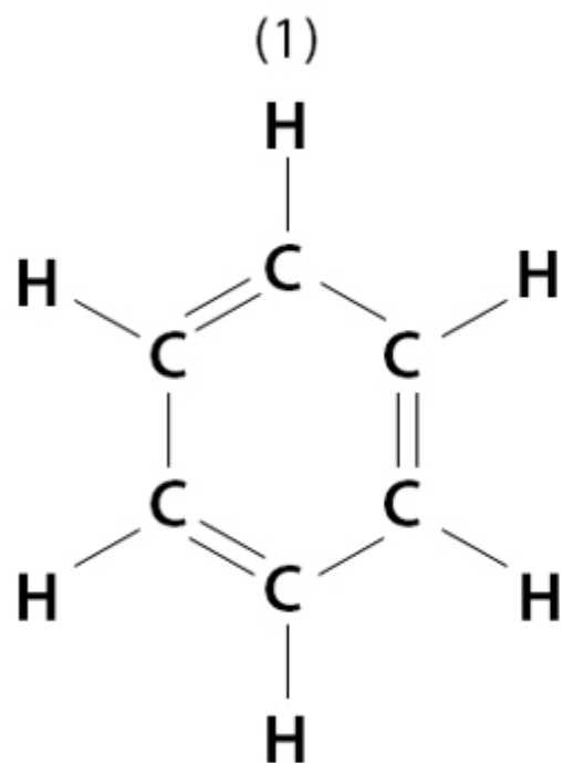
Lewis structure
